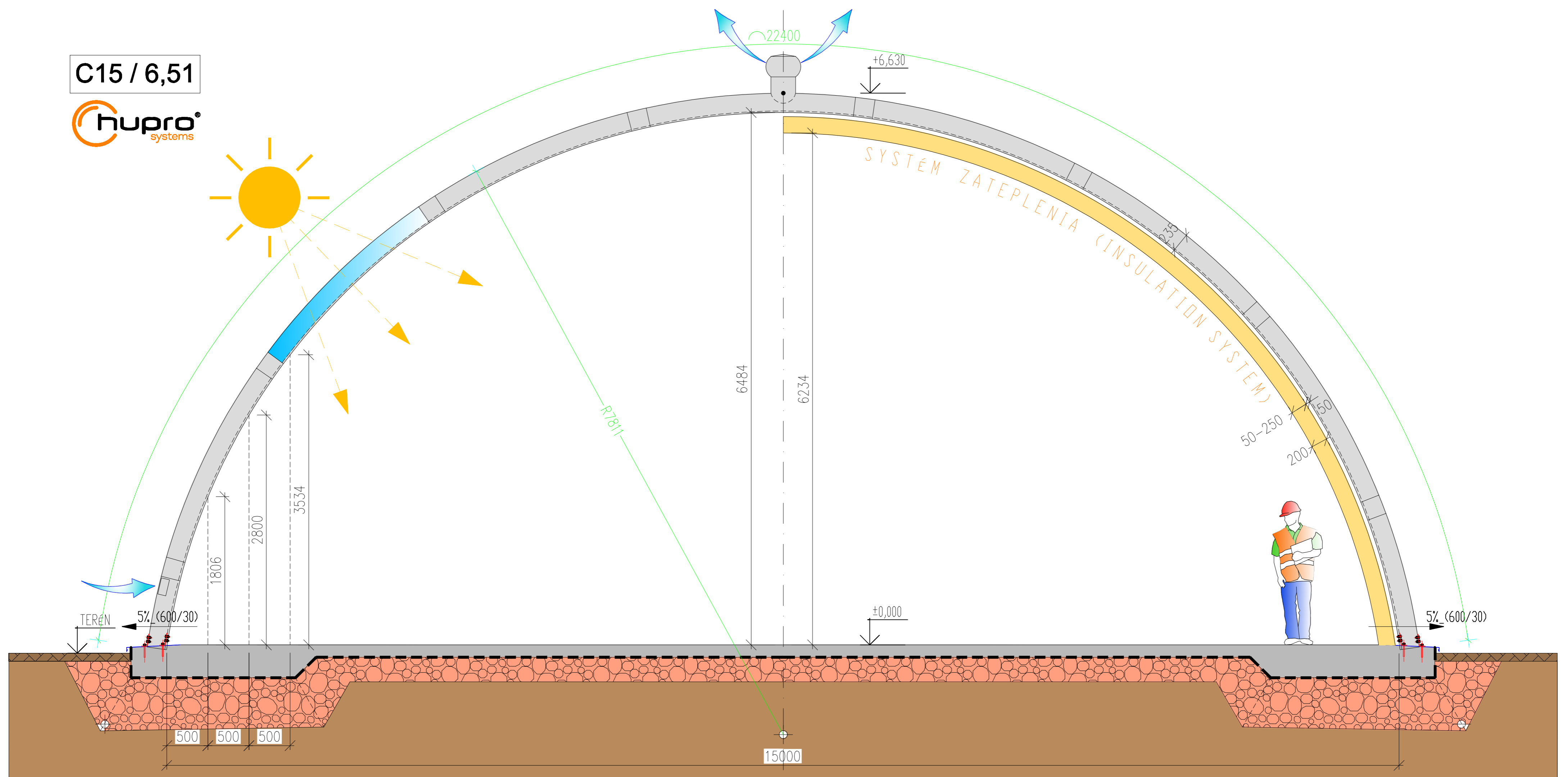
ORIENTAČNÝ TVAR ZAKLADANIA (ORIENTATION FORM OF FOUNDING)
